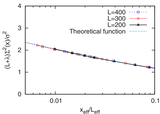
FIG. 3. (Color online) The same plot in Fig. 2 resolved more at the left-hand boundary of the model and taking the x axis in logarithmic scale.
