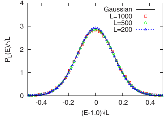
FIG. 1. (Color online) Scaling collapse of the probability distribution \mathcal{P}_L(E) of energy per site in the steady state for different systems of size 200, 500, and 1000. The distribution is well described by a Gaussian of width 0.136.
