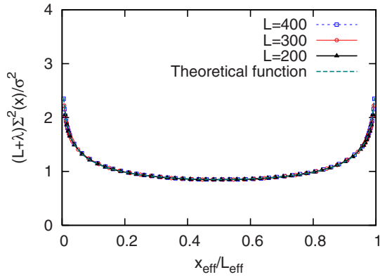
FIG. 2. (Color online) Scaling collapse of \Sigma^2(x)/\sigma^2 at site x for systems of different length L .
